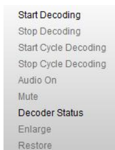
Figure 5.15 Start Decoding
