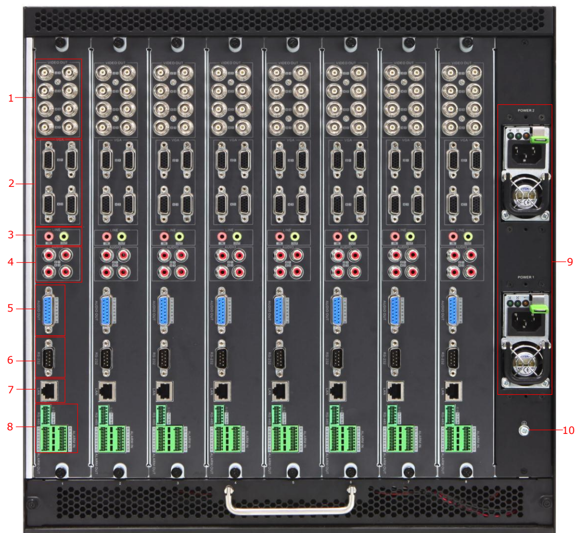
Figure 2.3 Rear Panel
