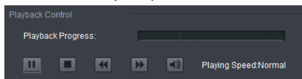
Figure 4.42 Playback Control
