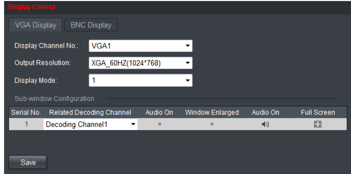
Figure 4.3 Display Configure
