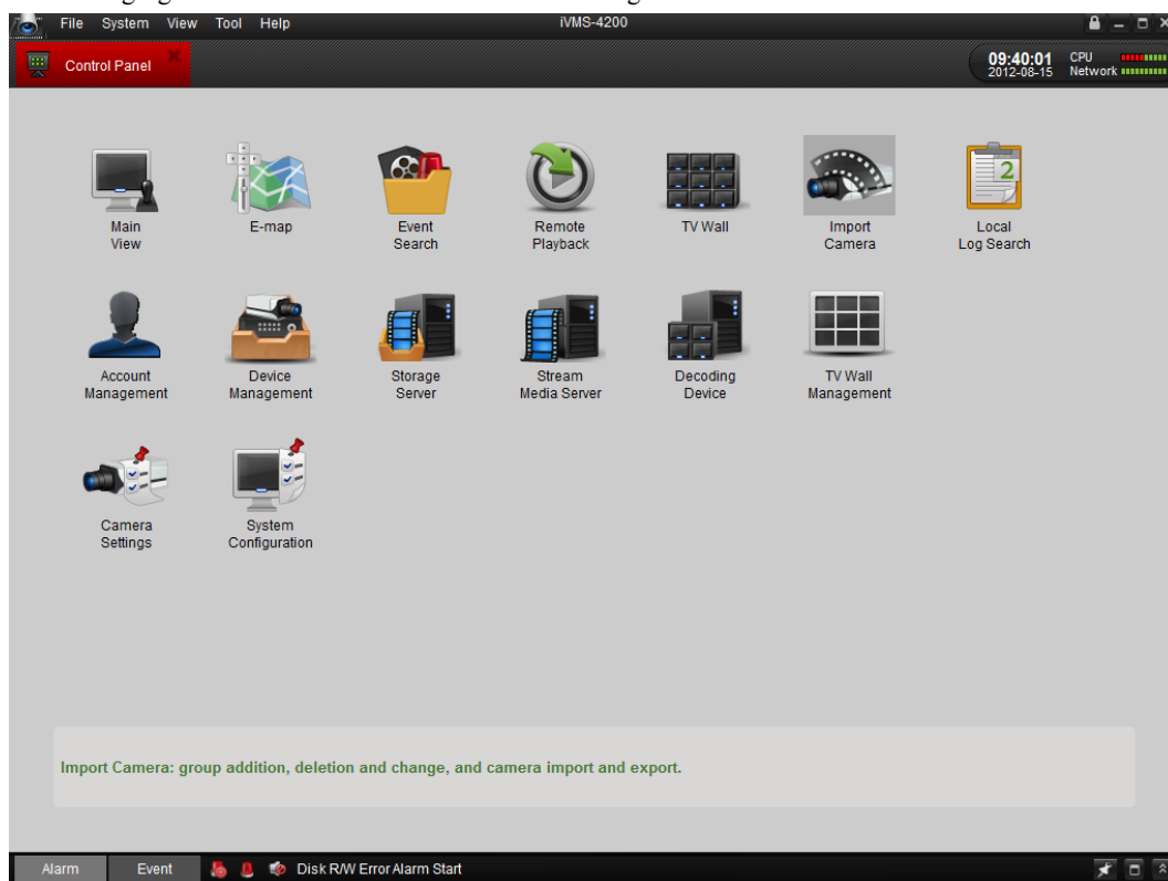
Figure 5.1 Control Panel
