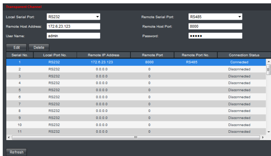
Figure 4.20 Check Connecting Status of Transparent Channel
