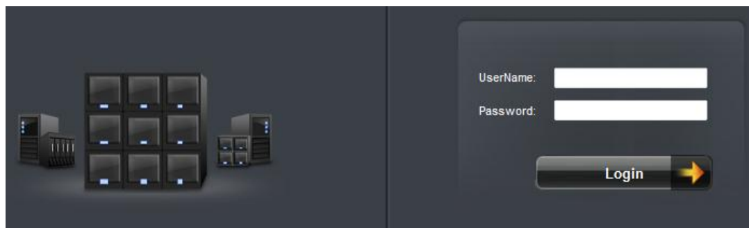
Figure 4.1 Login Interface
