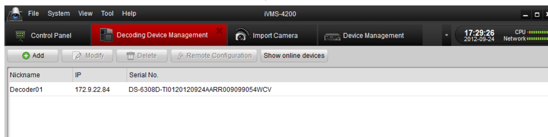
Figure 5.16 Decoder List
