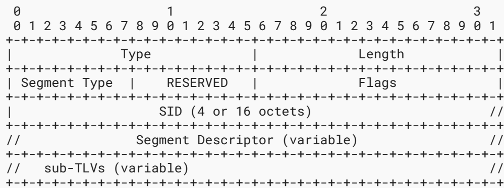
Figure 19: SR Segment Sub-TLV Format
