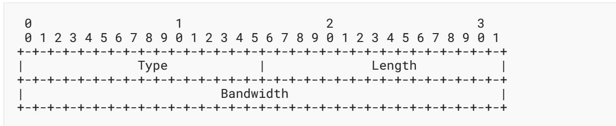
Figure 14: SR Bandwidth Constraint Sub-TLV Format
